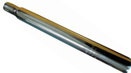
Espigão Selim 300mm 28.6 REF.: 50.206.1 – Cromado
