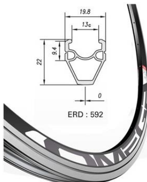
Aro 700C Mach 1 OMEGA 32 Furos
